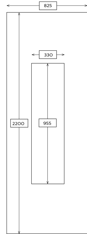
Gas input 15kW/hr (NG or LPG) Approximate weight 250 kg
